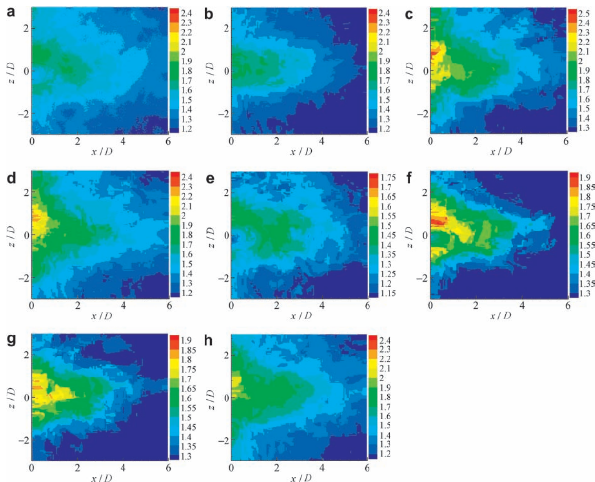
Fig. 5. Heat transfer coefficient h_g/h_0 at Re_D = 3191 and Rt = 0 . (a) Air injection, M = 0.4 ; (b) air injection, M = 0.8 ; (c) air injection, M = 1.2 ; (d) air injection, M = 1.6 ; (e) CO_2 injection, M = 0.4 ; (f) CO_2 injection, M = 0.8 ; (g) CO_2 injection, M = 1.2 ; and (h) CO_2 injection, M = 1.6 .
