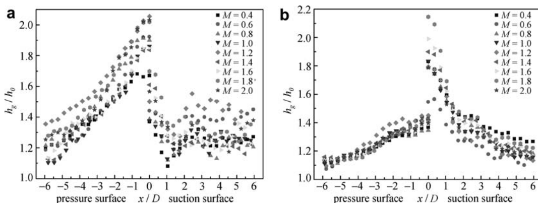
Fig. 8. Laterally averaged heat transfer coefficient h_g/h_0 at Re_D = 3191 and Rt = 0.0249 . (a) Air injection and (b) CO_2 injection.
