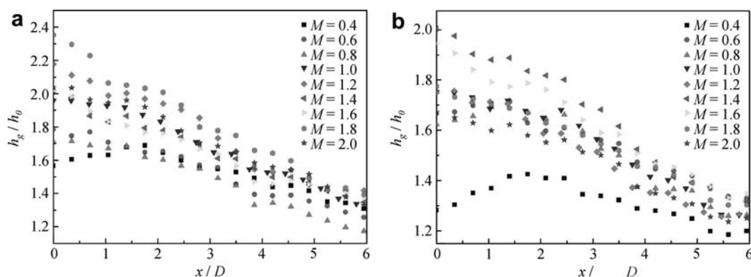
Fig. 6. Laterally averaged heat transfer coefficient h_g/h_0 at Re_D = 3191 and Rt = 0 . (a) Air injection and (b) CO_2 injection.
